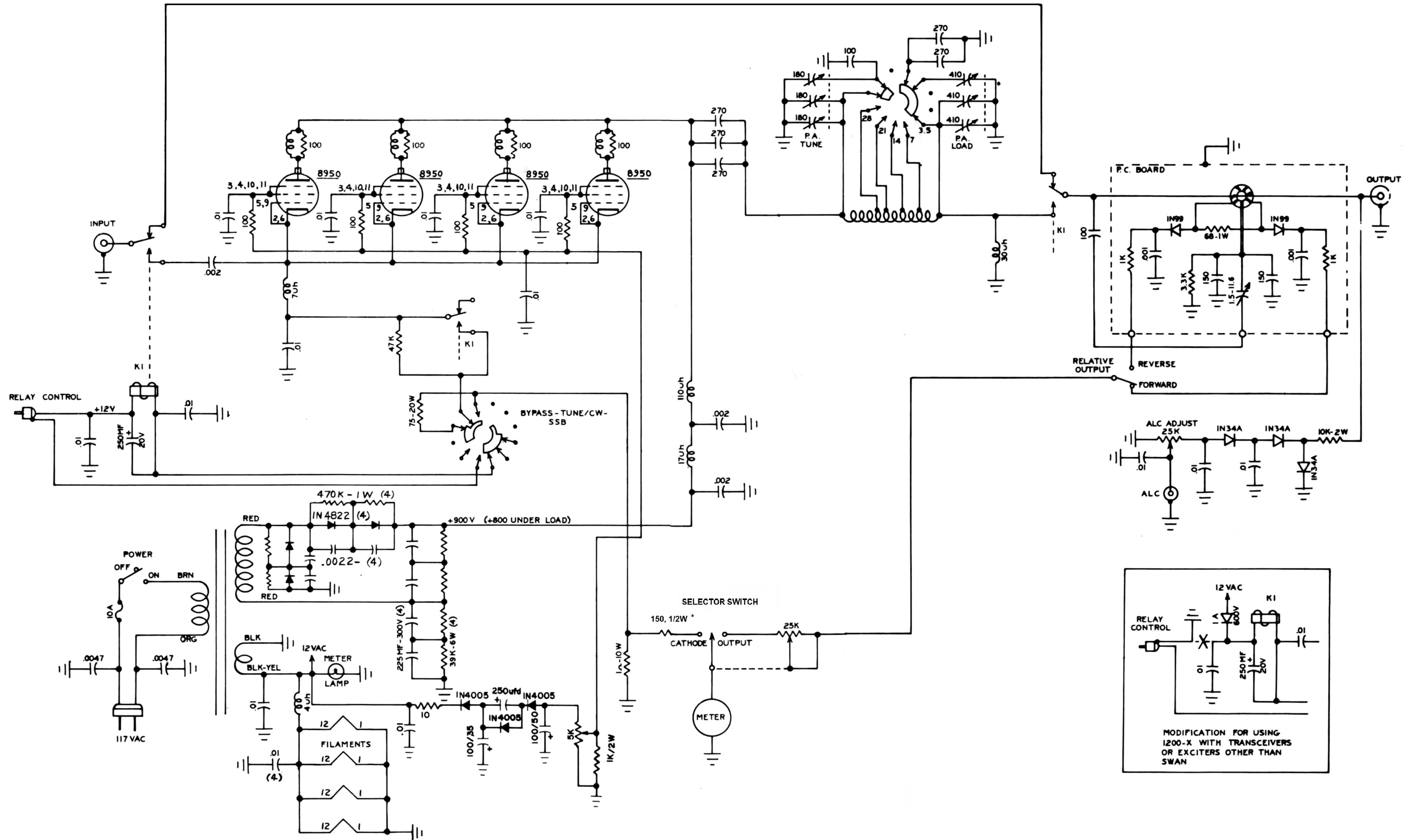
Swan Model 1200-X Cynet Linear Amplifier Schematic Diagram
